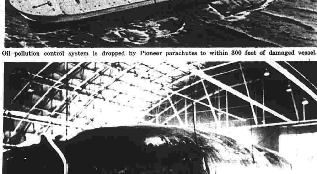
Bladder, being assembled by Pioneer at Bradley Field, is shown in its inflated, 140-foot length.
